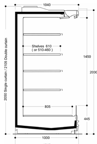
LARGE - H20
