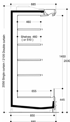
NARROW - H20
