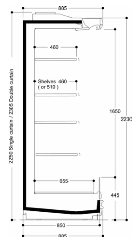
NARROW - H22
