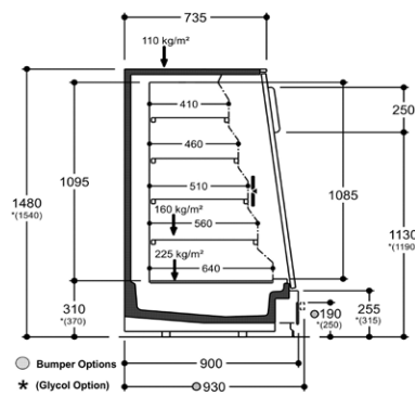
NARROW - H15 TILTED DOORS
