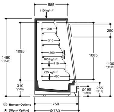
COMPACT - H15 TILTED DOORS
