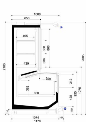
H2000 - LG300
