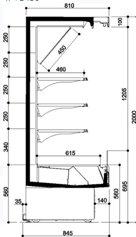
4P+S450
