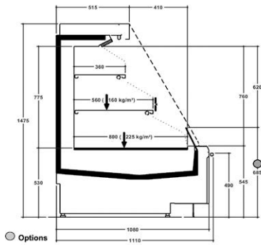
15 LARGE - DESIGN
