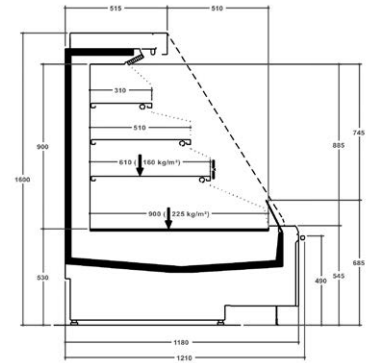
16 XL - DESIGN
