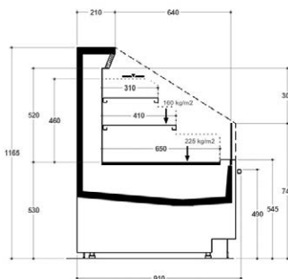
12 NARROW - DESIGN
