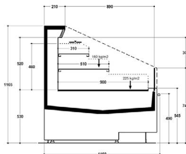
12 XL - DESIGN
