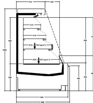
16 NARROW - DESIGN
