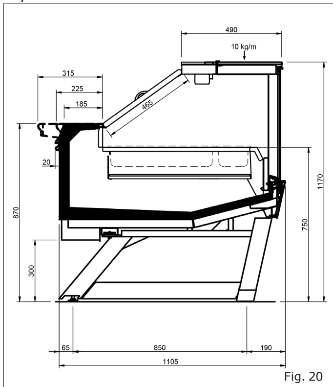
Style RDB with feet
