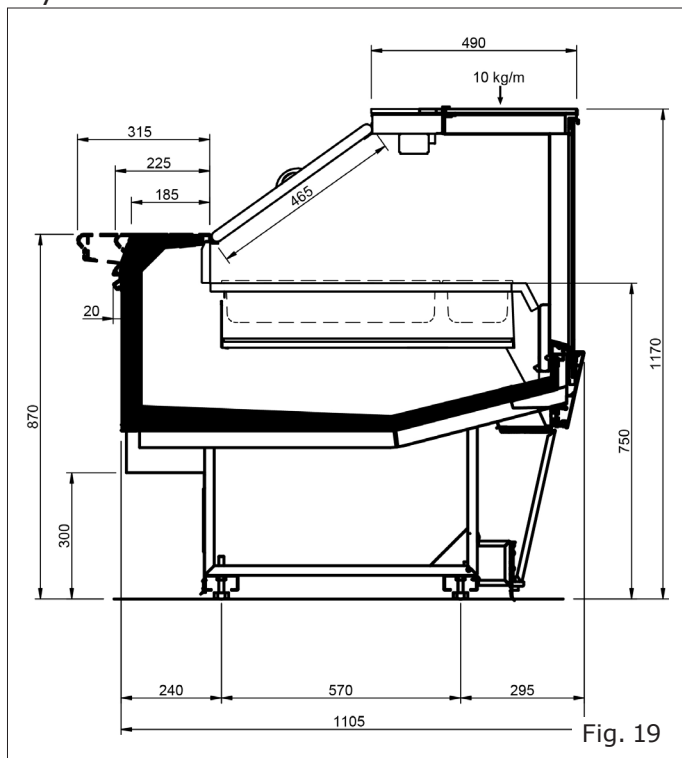
Style RDB with feet
