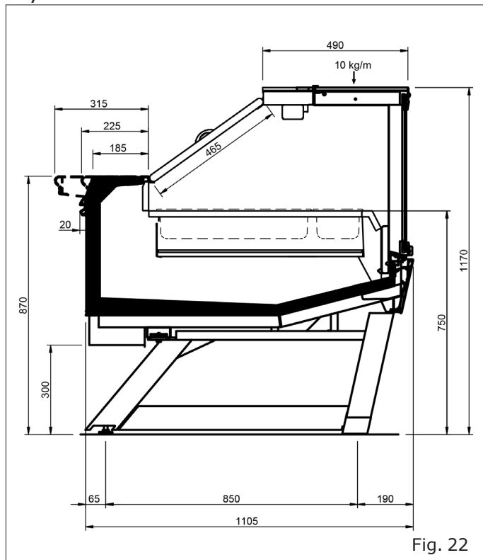
Style WO with feet
