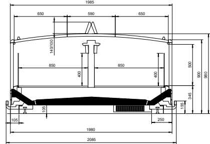
NordicLine IS7 200-90 curved lids
